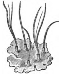
FIG. 342. — Anthoceros lewisii , natural size.
